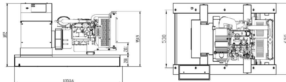
Open Type ( without Soundproof Canopy)
