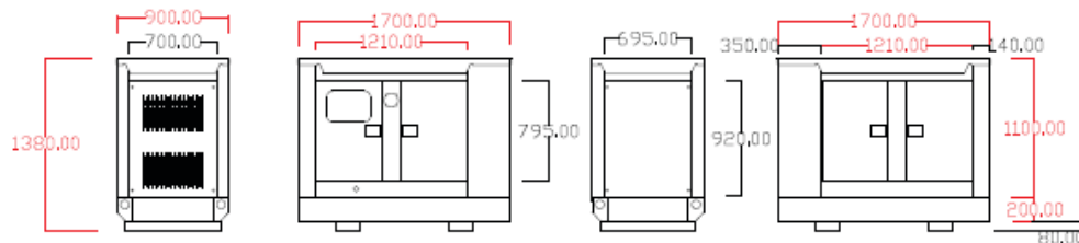
Open Type ( without Soundproof Canopy)
